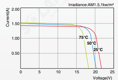
SLP020-12 I-V Curves
